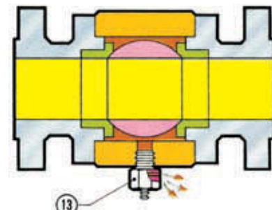
OPEN VALVE
