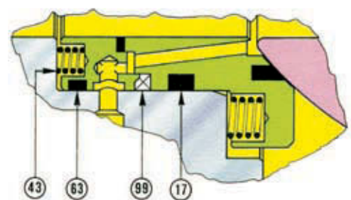
Fire Safe Seat BS 6755
