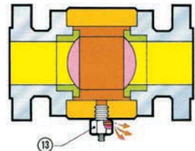
CLOSED VALVE
