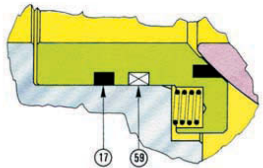
Fire Safe Seat API 607
