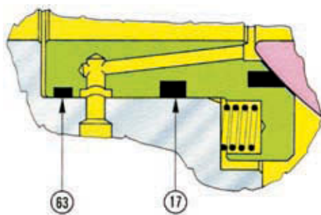
Seat sealing
